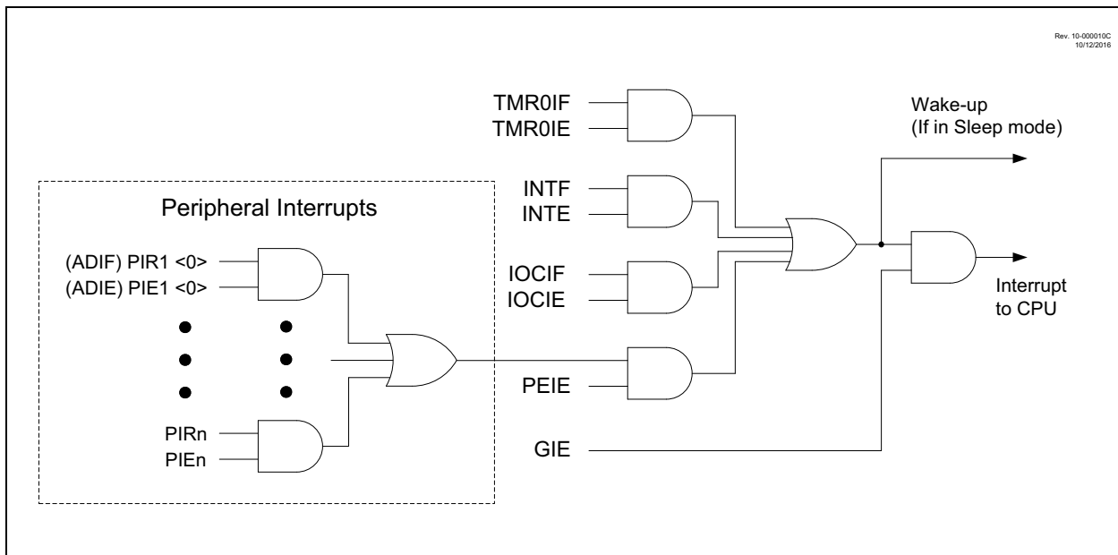
FIGURE 10-1: INTERRUPT LOGIC
