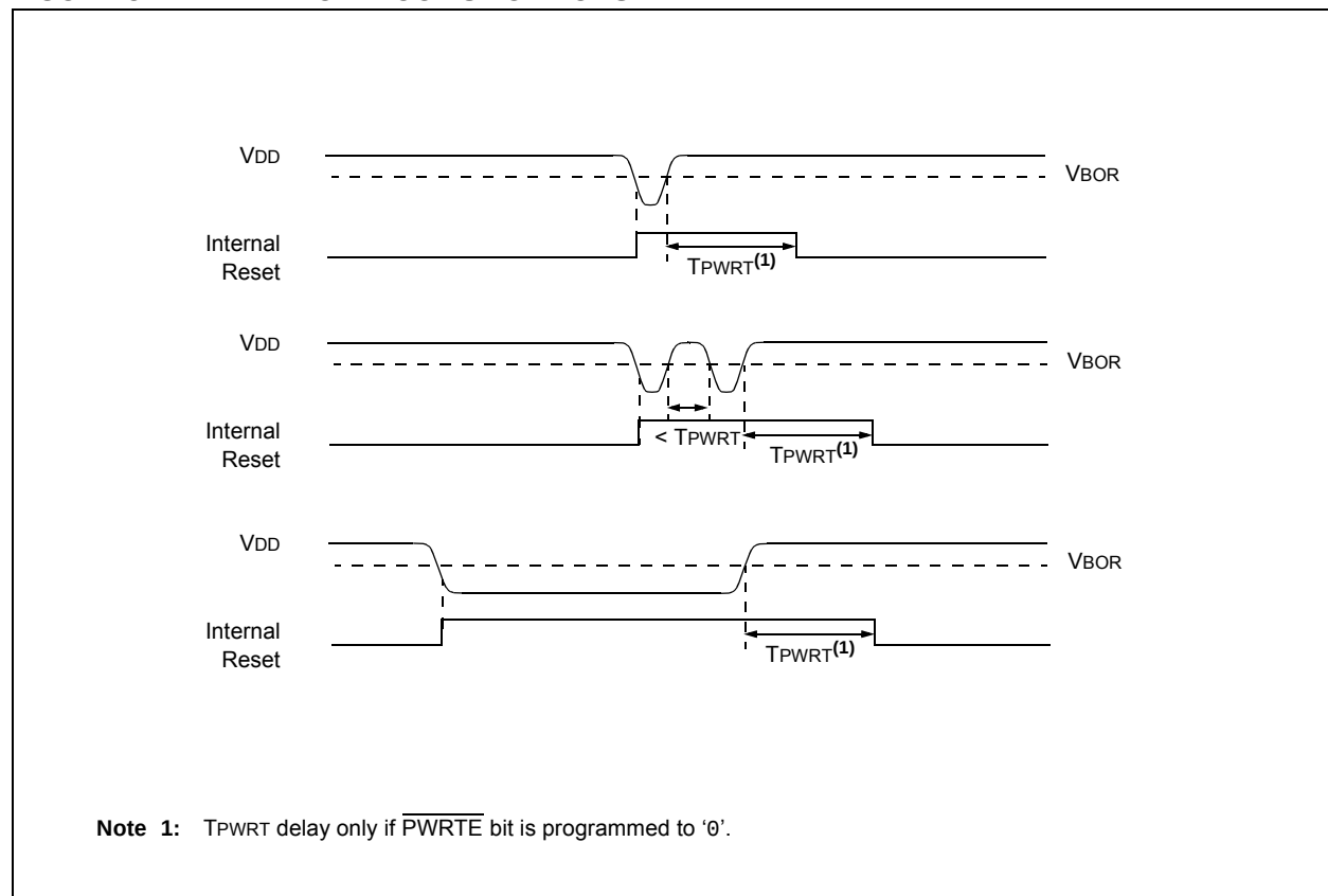
FIGURE 8-2: BROWN-OUT SITUATIONS
