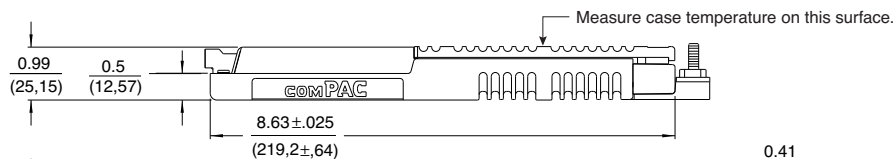
Standard Heat sink
