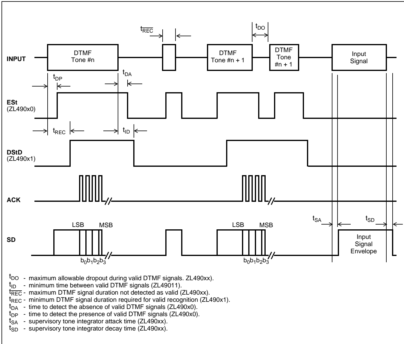
Figure 4 - Timing Diagram
