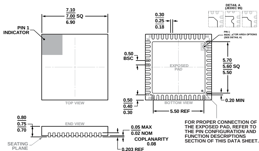
Figure 66. 48-Lead Lead Frame Chip Scale Package [LFCSP] 7 mm x 7 mm Body and 0.75 mm Package Height (CP-48-13)
