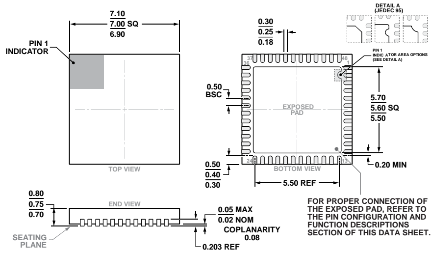
Figure 66. 48-Lead Lead Frame Chip Scale Package [LFCS] 7 mm x 7 mm Body and 0.75 mm Package Height (CP-48-13) Dimensions shown in millimeters
