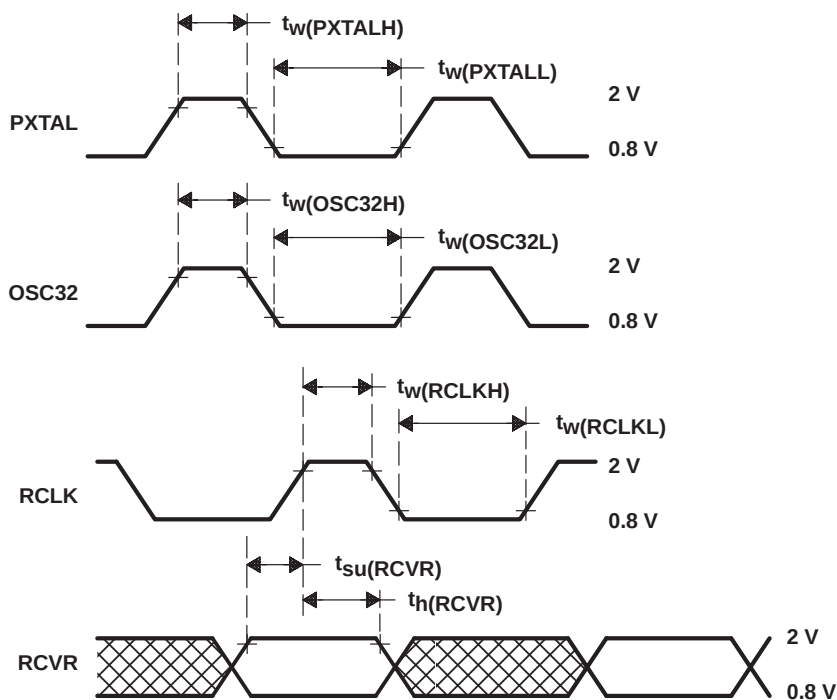
Figure 8. PXTAL, OSC32, RCLK, and RCVR
