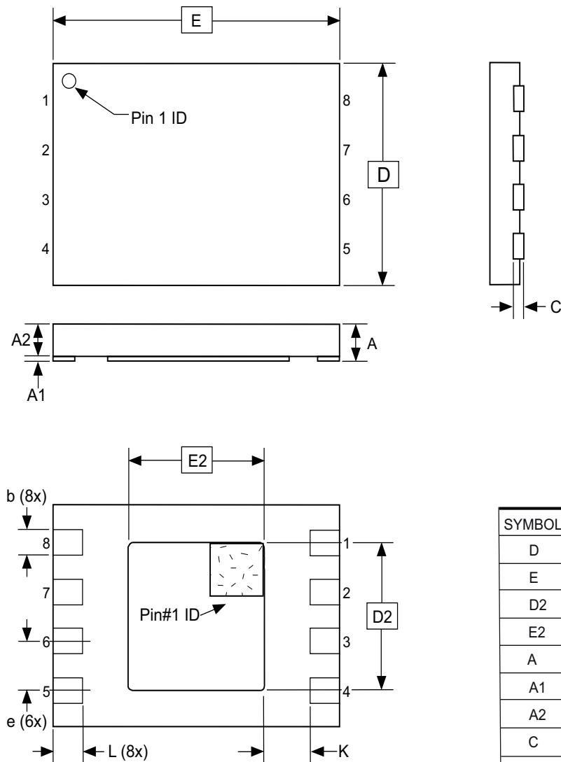
COMMON DIMENSIONS (Unit of Measure = mm)
