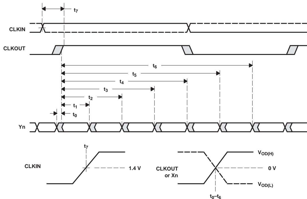
Figure 5. Timing Definitions
