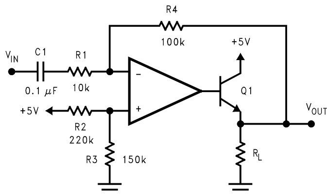
Figure 70. Power Amplifier
