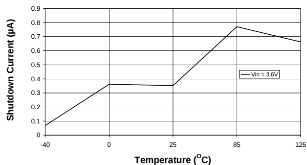
Shutdown Current vs Temperature
