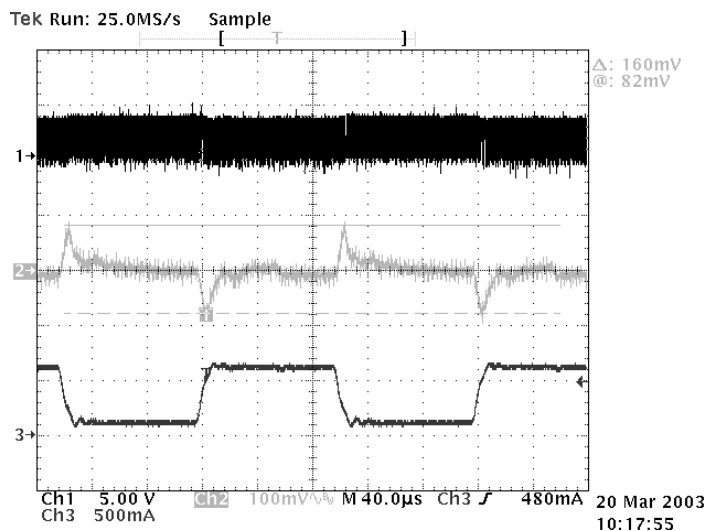
PWM, Cout = 10uF, Lout = 10uH
