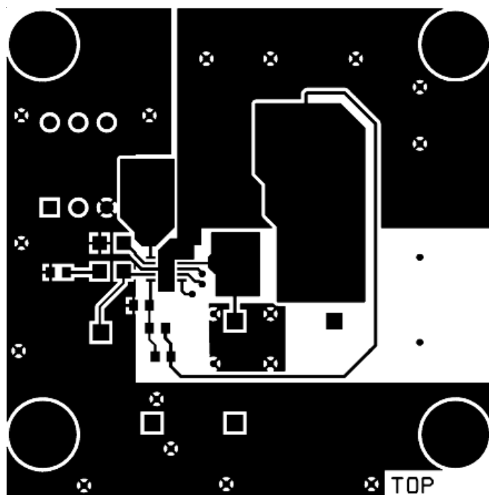
TOP COPPER
