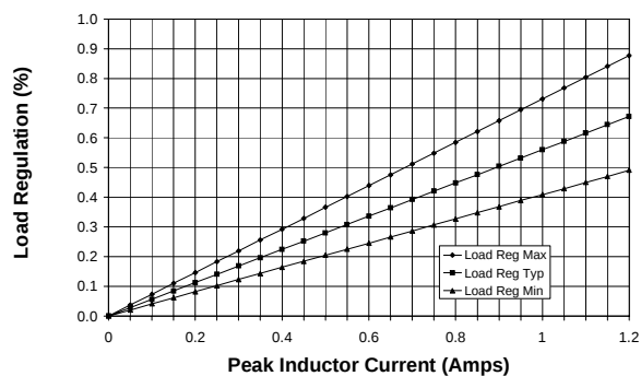
SC192 Load Regulation Limits
