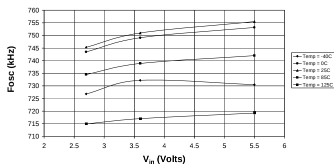
Oscillator Frequency vs V_{IN} Over Temperature
