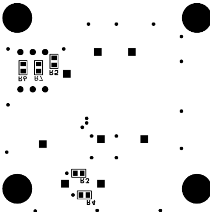
BOTTOM SILKSCREEN
