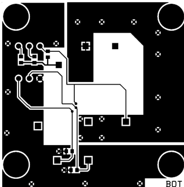
BOTTOM COPPER
