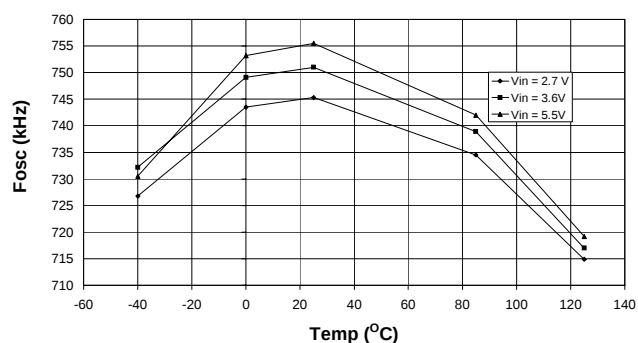
Oscillator Frequency vs Temperature Over V_{IN}
