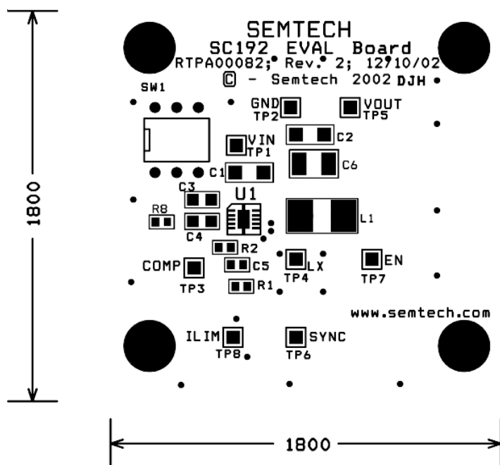
TOP SILKSCREEN
