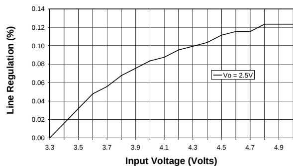
Line Regulation at I_{OUT} = 300mA
