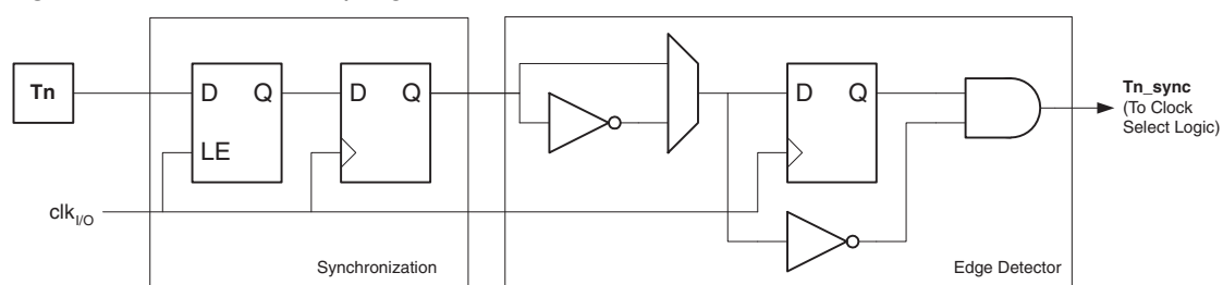
Figure 12-1. T0 Pin Sampling
