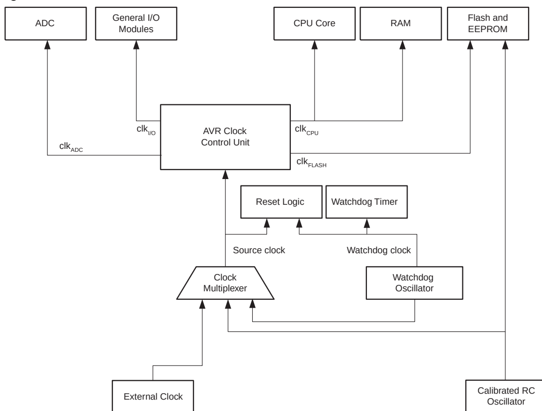
Figure 6-1. Clock Distribution
