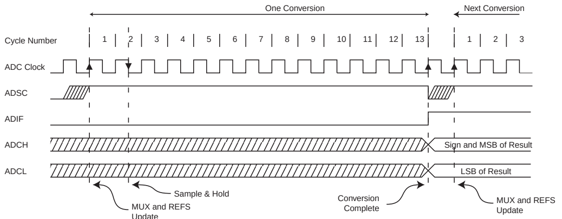
Figure 14-5. ADC Timing Diagram, Single Conversion
