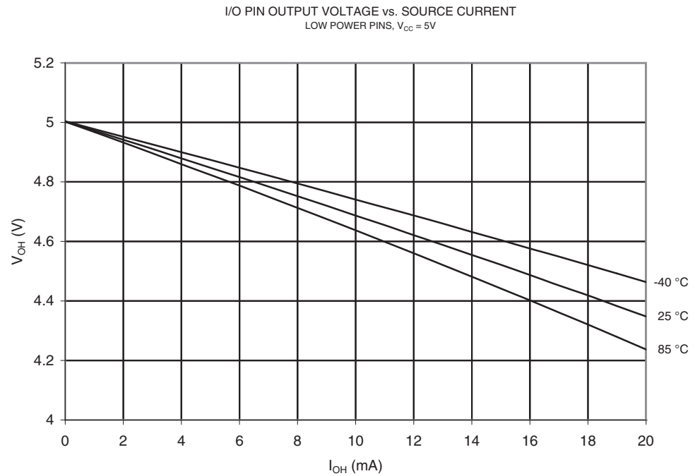
Figure 19-29. V_{OH} : I/O Pin Output Voltage vs. Source Current (Low Power Pins, V_{CC} = 5V )
