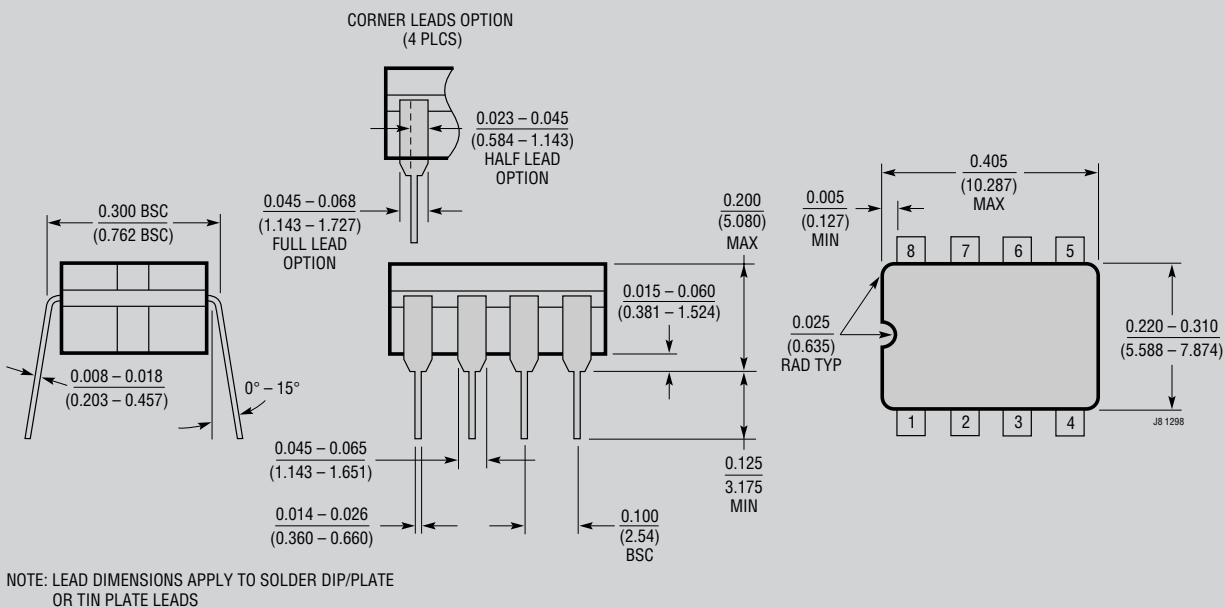
J8 Package 8-Lead Cerdip (Narrow .300 Inch, Hermetic) (Reference LTC DWG # 05-08-1110)
