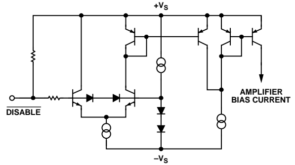
Figure 70. \overline{DISABLE} Pin Circuit
