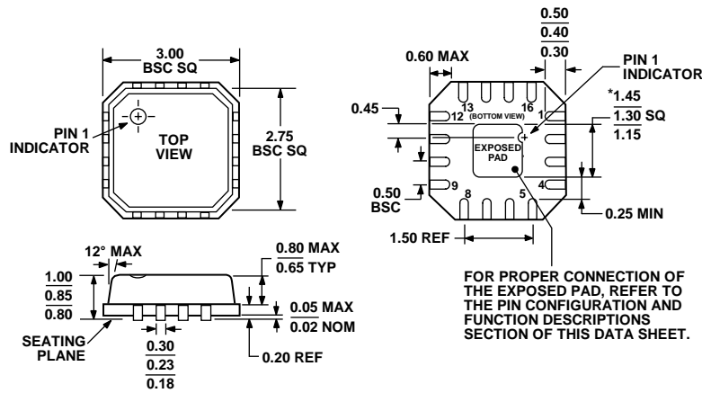
*COMPLIANT TO JEDEC STANDARDS MO-220-VEED-2 EXCEPT FOR EXPOSED PAD DIMENSION. Figure 77. 16-Lead Lead Frame Chip Scale Package [LFCSP_VQ] 3 mm x 3 mm Body, Very Thin Quad (CP-16-2) Dimensions shown in millimeters
