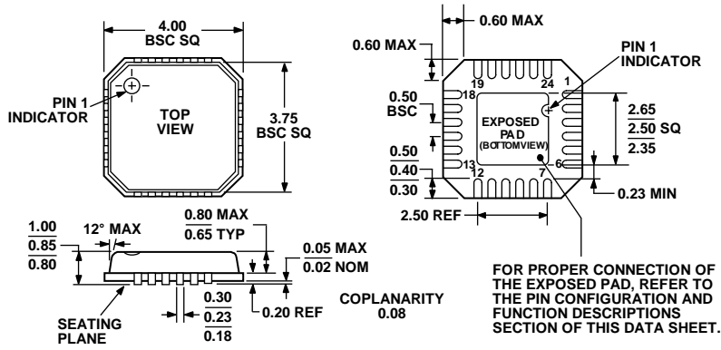
Figure 79. 24-Lead Lead Frame Chip Scale Package [LFCSP_VQ] 4 mm × 4 mm Body, Very Thin Quad (CP-24-3) Dimensions shown in millimeters
