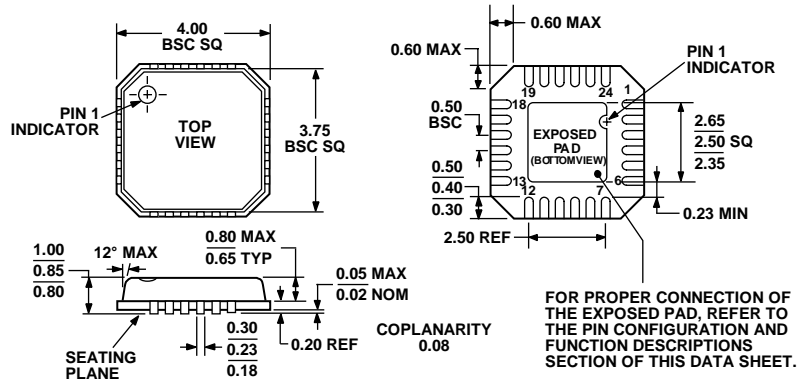
Figure 79. 24-Lead Lead Frame Chip Scale Package [LFCSP_VQ] 4 mm x 4 mm Body, Very Thin Quad (CP-24-3) Dimensions shown in millimeters
