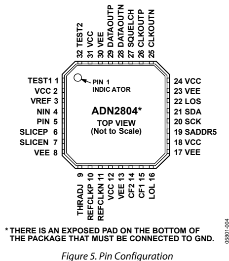
Figure 5. Pin Configuration
