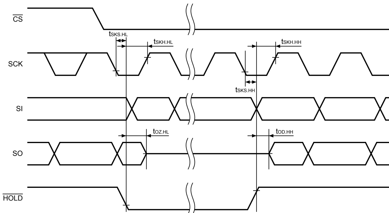
Figure 5 Hold Timing
