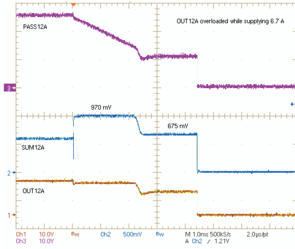
Figure 22. OUT12A Overloaded While Supplying 6.7 A
