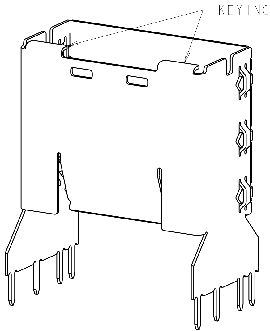
1888413-6 SCALE 5:1
