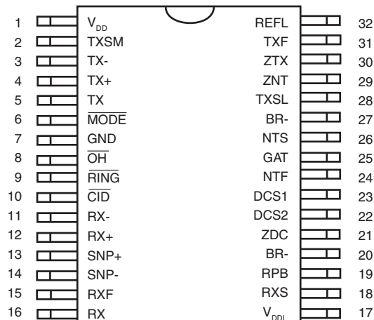
Figure 1. Pinout
