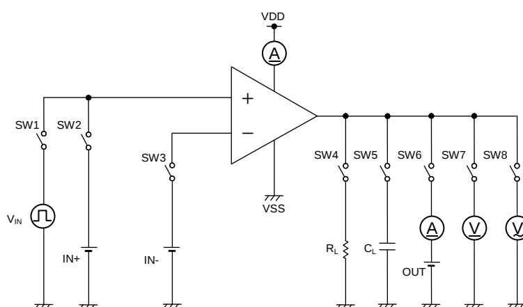
Figure 24. Test Circuit 2
