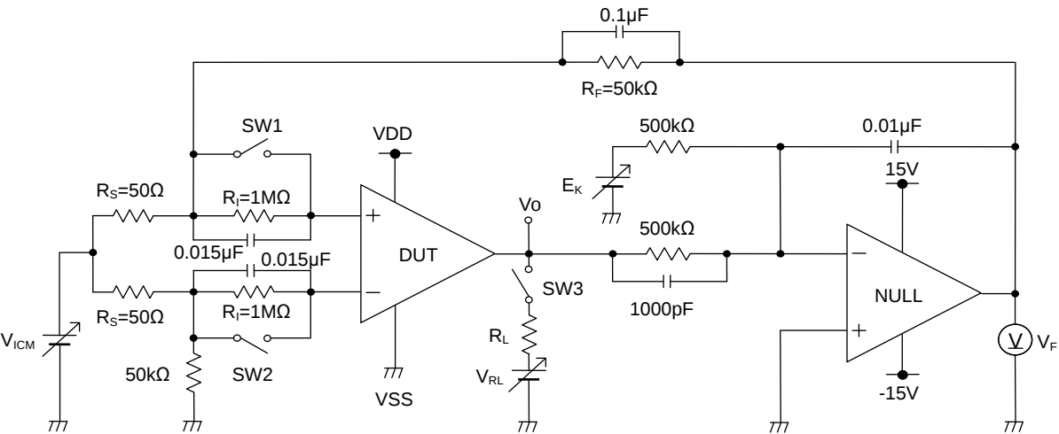
Figure 23. Test Circuit 1
