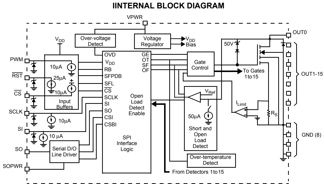
Figure 2. 33996 Simplified Internal Block Diagram
