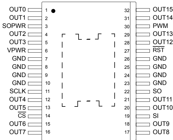
Figure 3. 33996 Pin Locations
