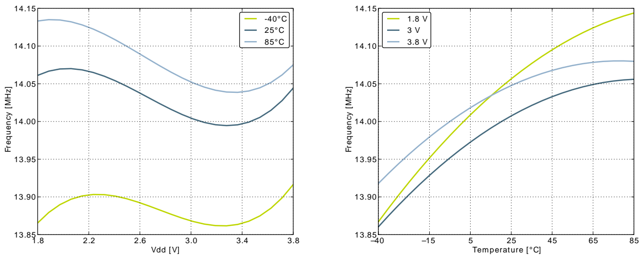
Figure 3.24. Calibrated HFRCO 21 MHz Band Frequency vs Temperature and Supply Voltage
