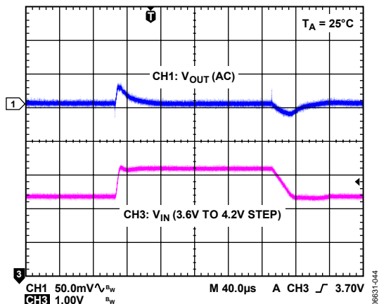
Figure 37. Line Transient Response ( V_{OUT} = 1.8 V )
