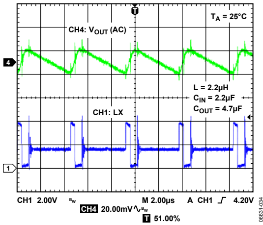
Figure 41. PSM Mode Ripple (V IN = 3.6 V, Load = 50 mA)
