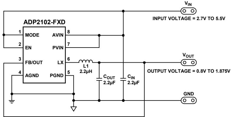
Figure 47. ADP2102-FXD ( 0 \text{ mA} \leq I_{LOAD} \leq 300 \text{ mA} )
