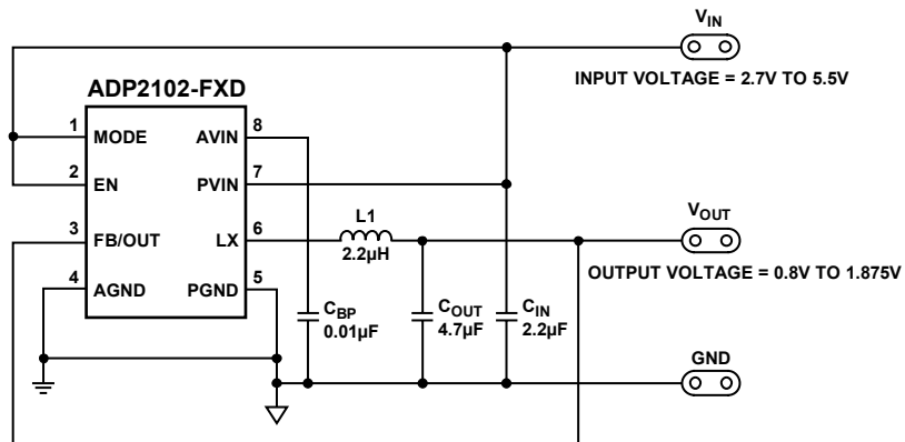
Figure 48. ADP2102-FXD ( 0 \text{ mA} \leq I_{LOAD} \leq 600 \text{ mA} )
