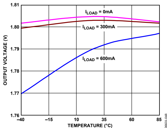
Figure 17. Output Voltage vs. Temperature ( V_{OUT} = 1.8\text{ V} )
