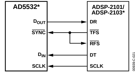
Figure 22. AD5532 to ADSP-2101/ADSP-2103 Interface
