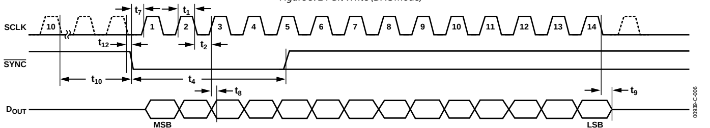
Figure 6. 14-Bit Read (Both Readback Modes)
