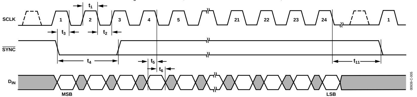
Figure 5. 24-Bit Write (DAC Mode)
