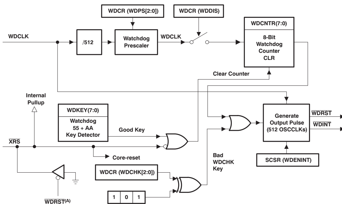
Figure 2-16. CPU-Watchdog Module
