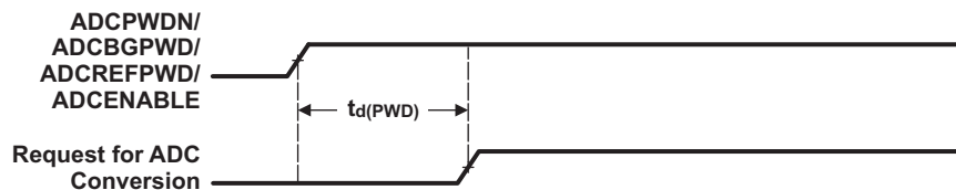
Figure 5-17. ADC Conversion Timing
