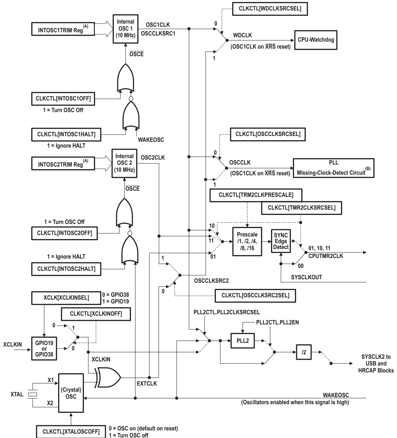
Figure 2-12. Clock Tree
