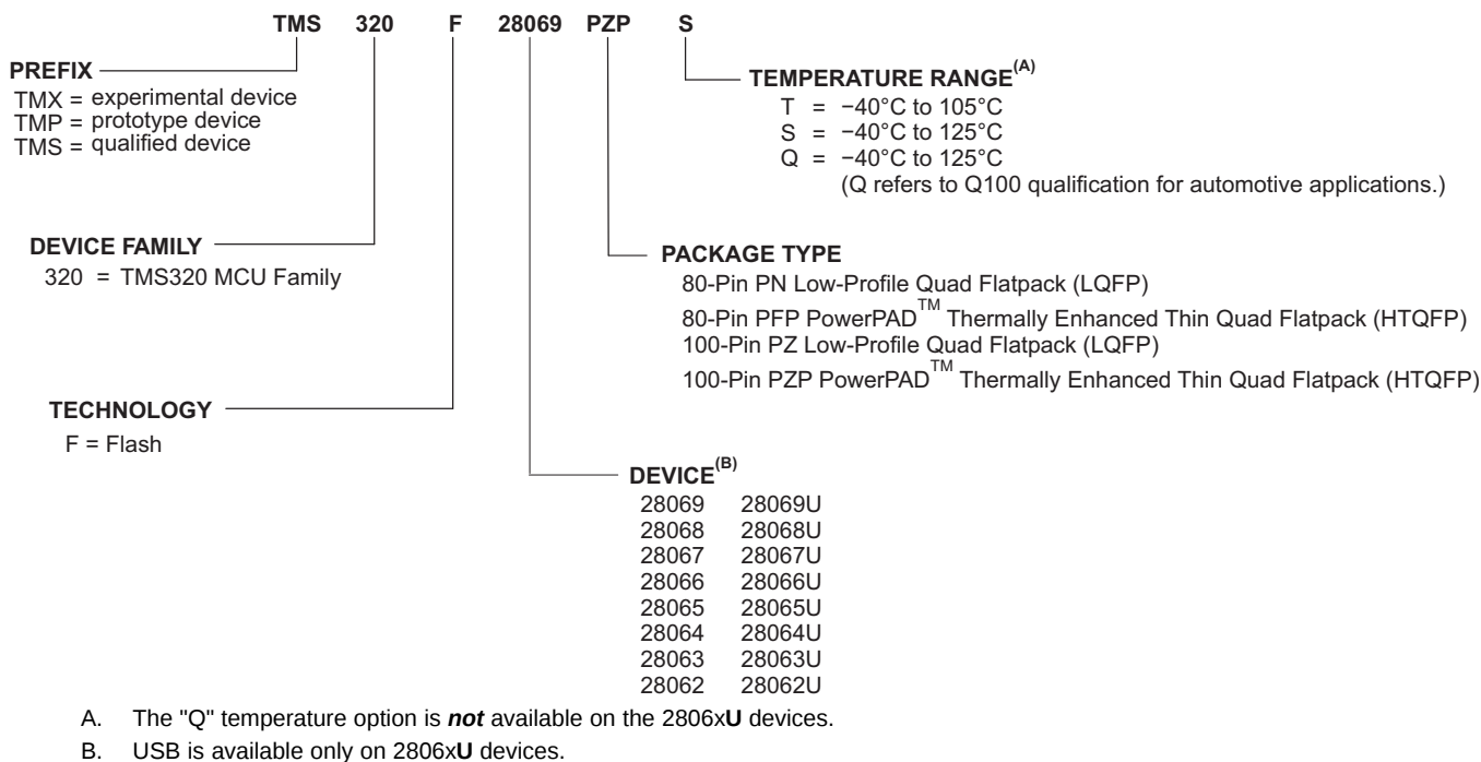
Figure 3-1. Device Nomenclature
