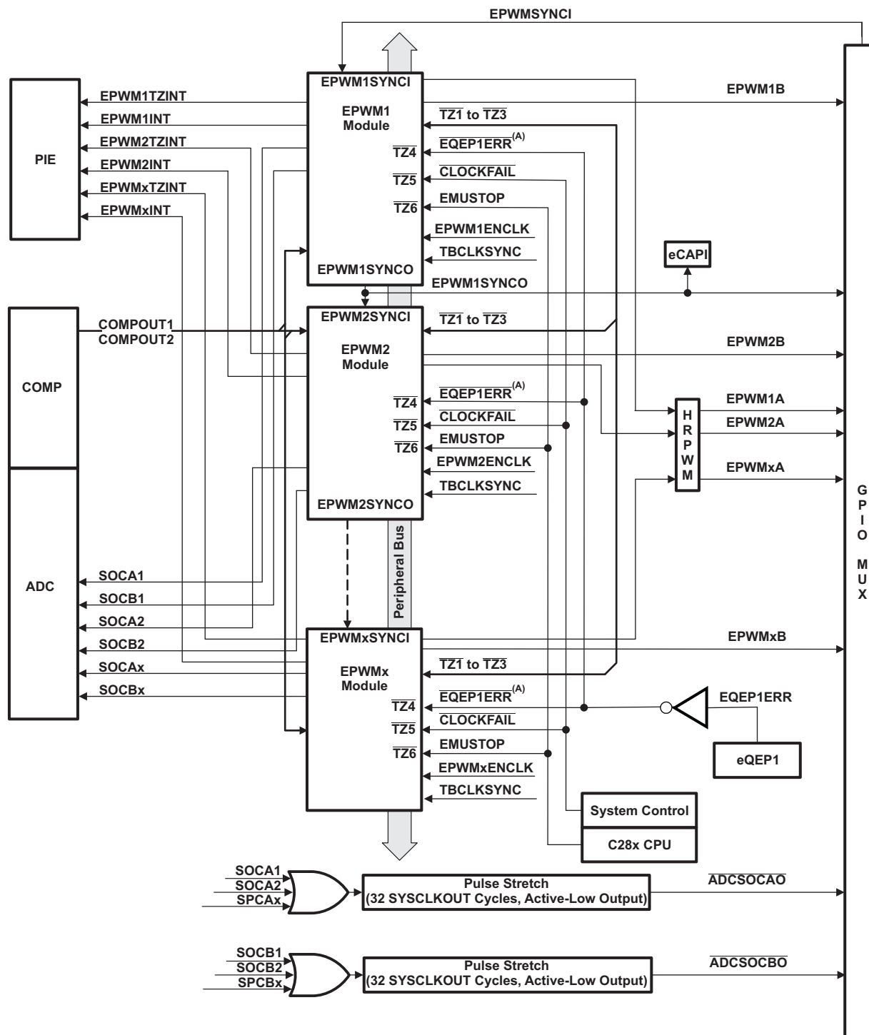
Figure 5-42. ePWM
