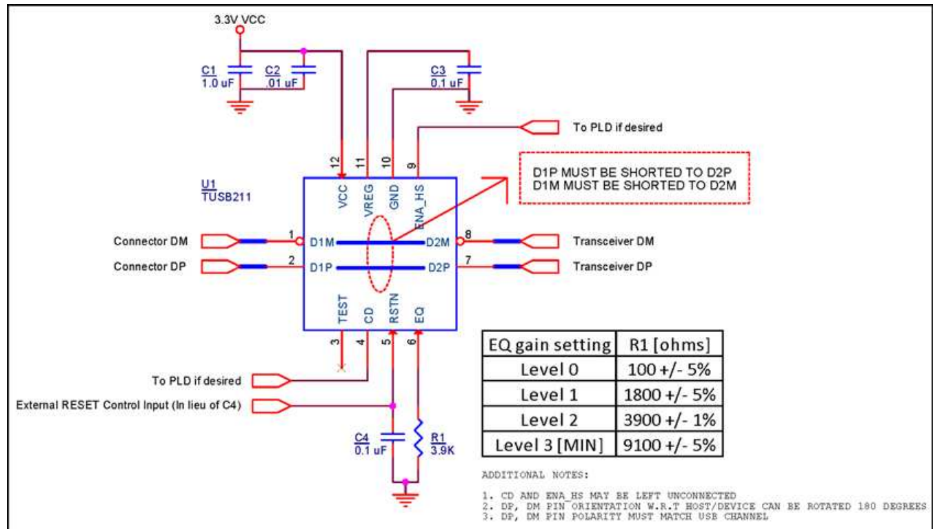
Figure 1. Reference Schematic
