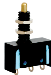
Telescopic plunger with 3 mm overtravel and with M6 x 0.75 threaded barrel
