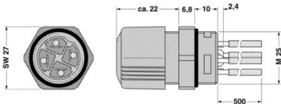
Dimensioned drawing
