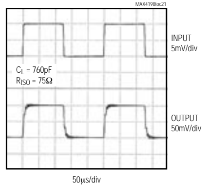
MAX4199 SMALL-SIGNAL PULSE RESPONSE WITH EXCESSIVE CAPACITIVE LOAD AND ISOLATION RESISTOR
