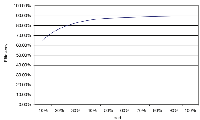
Figure 16 EMA212PS48
