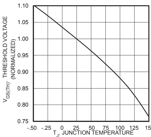
FIGURE 7, Threshold Voltage vs Junction Temperature
