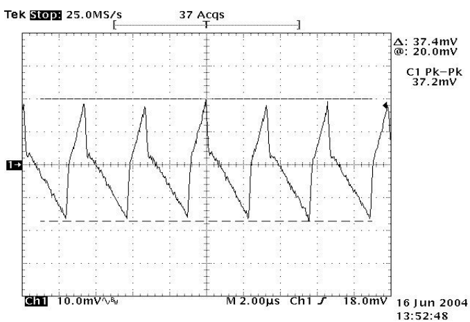
Figure 11: Output ripple & noise at 12Vin, 3.3V/15A out
