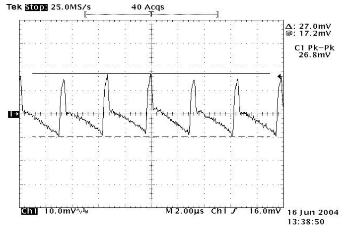
Figure 8: Output ripple & noise at 12Vin, 1.2V/15A out
