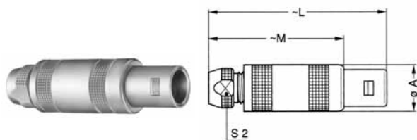
Reference Dimensions (mm) Model Series A L M S2 FFA 00 ✓ 6.4 26.0 18.0 4.5 FFA 0S ✓ 9.0 34.5 24.5 6.5 FFA 1S ✓ 12.0 42.5 31.5 8.5 FFA 2S ✓ 14.8 52.0 40.0 11.0 FFA 3S ✓ 17.8 61.0 46.0 14.0 FFA 4S ✓ 24.8 77.0 59.0 19.0 FFA 5S ✓ 35.1 103.0 78.0 29.0
