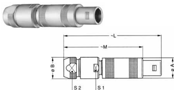
Reference Dimensions (mm) Model Series A B L M S1 S2 FFA 00 ✓ 6.4 8.0 34.0 26.0 7.0 6.5 FFA 0S ✓ 9.0 10.0 45.5 35.5 9.0 8.5 FFA 1S ✓ 12.0 13.0 57.0 46.0 12.0 11.0 FFA 2S ✓ 14.8 18.0 67.0 55.0 14.0 14.0 FFA 3S ✓ 17.8 21.0 85.0 70.0 19.0 19.0 FFA 4S ✓ 24.8 31.8 107.0 89.0 28.5 29.0 FFA 5S ✓ 35.1 41.8 138.0 113.0 37.5 38.0
