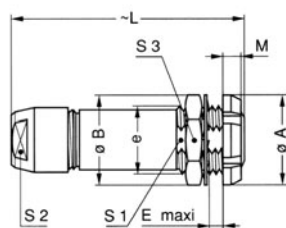
Reference Dimensions (mm) Model Series A B e E L M S1 S2 S3 PFG 1B ✓ 16 16 M12x1.0 5.0 40.5 3.5 10.5 9 14 PFG 2B ✓ 20 20 M15x1.0 6.5 47.0 3.5 13.5 12 17 PFG 3B ✓ 24 25 M18x1.0 9.0 56.0 4.5 16.5 14 22 PFG 4B ✓ 30 32 M25x1.0 11.0 73.0 4.5 23.5 20 30
