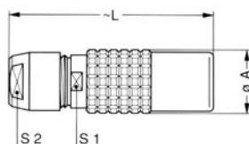
Reference Dimensions (mm) Model Series A L S1 S2 PHG 1B ✓ 12.5 40.5 10 9 PHG 2B ✓ 16.5 47.0 13 12 PHG 3B ✓ 19.0 56.0 15 14 PHG 4B ✓ 24.4 73.0 21 20 PHG 5B ✓ 34.2 99.0 31 30
