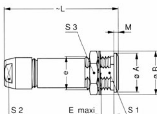
Reference Dimensions (mm) Model Series A B e E L M S1 S2 S3 PKG 1B ✓ 14 16.0 M12x1.0 7.5 40.5 1.5 10.5 9 14 PKG 2B ✓ 18 19.5 M15x1.0 8.5 47.0 1.8 13.5 12 17 PKG 3B ✓ 22 25.0 M18x1.0 11.5 56.0 2.0 16.5 14 22 PKG 4B ✓ 28 32.0 M25x1.0 12.5 73.0 2.5 23.5 20 30 PKG 5B ✓ 40 40.0 M35x1.0 11.0 99.0 3.0 33.5 30 -
