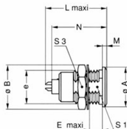
Reference Dimensions (mm) Model Series A B e E L M N S1 S3 EGG 1B ✓ 14 16 M12x1.0 7.5 21.7 1.5 19.5 10.5 14 EGG 2B ✓ 18 20 M15x1.0 8.5 25.0 1.8 21.5 13.5 17 EGG 3B ✓ 22 25 M18x1.0 11.5 30.0 2.0 25.5 16.5 22 EGG 4B ✓ 28 32 M25x1.0 12.0 34.5 2.5 30.5 23.5 30 EGG 5B ✓ 40 40 M35x1.0 15.5 45.5 3.0 36.5 33.5 -
