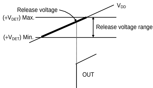
Figure 22 Release Voltage (CMOS Output Products)
