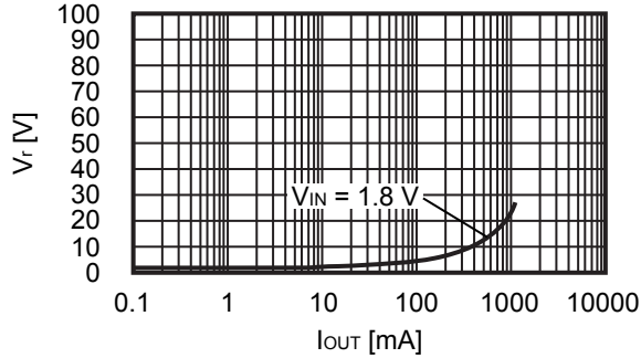
Condition 1 S-8365AABBA ( V_{OUT(S)} = 2.5 V )
