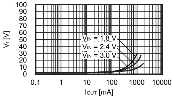
Condition 5 S-8365AABBA ( V_{OUT(S)} = 3.3 V )
