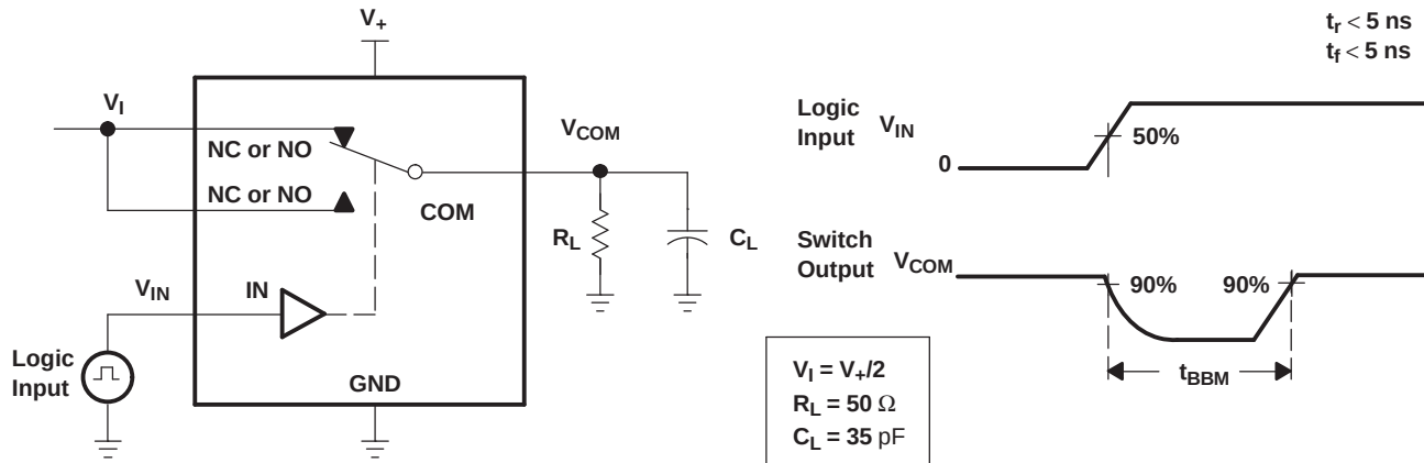
Figure 14. Break-Before-Make ( t_{\text{BBM}} ) Time
