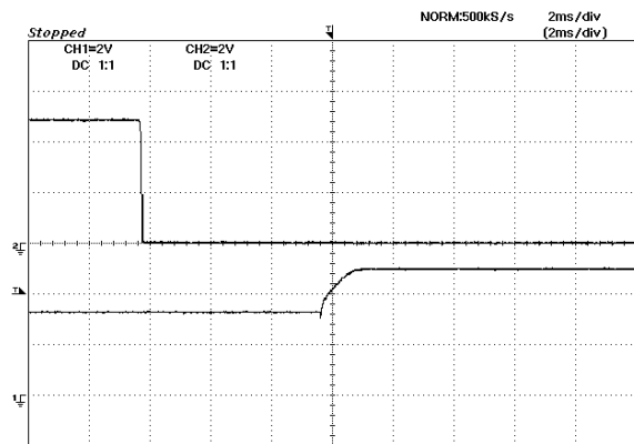
Figure 14: Typical transient response to step load change at 2.5\text{A}/\mu\text{s} from 50% to 100% of I_o , max at 12Vin, 5.0V out ( C_{out} = 1\mu\text{F} ceramic, 10\mu\text{F} tantalum) I_o: 2\text{A}/\text{DIV}
