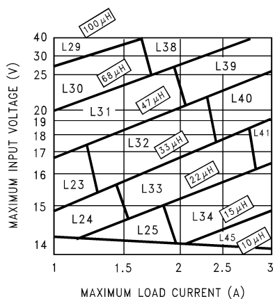
Figure 20. LM2673-12
