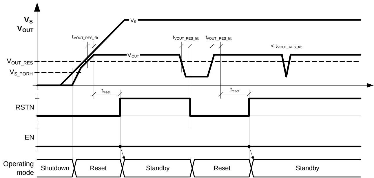
Figure 6. V OUT Regulator Voltage Monitoring
