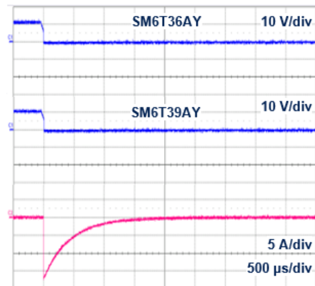
Figure 13. ISO7637-2 pulse 1: V_s = -150 V with 12 V battery
