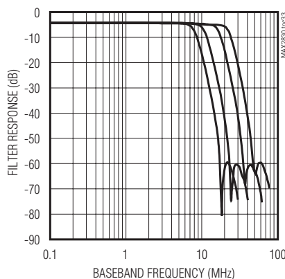
Tx BASEBAND FILTER RESPONSE
