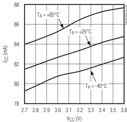
Tx I_{CC} vs. V_{CC}
