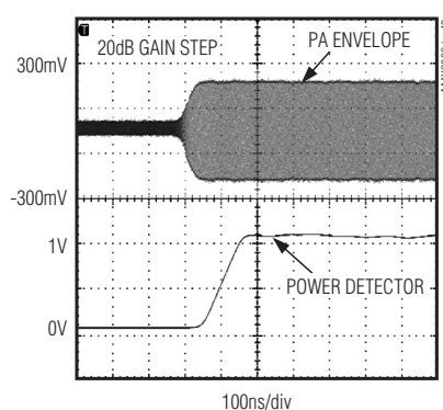
POWER-DETECTOR OUTPUT
