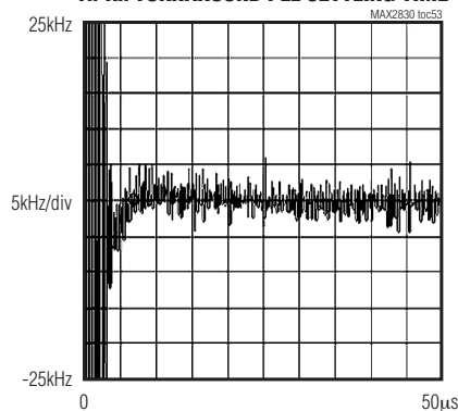
Tx-Rx TURNAROUND PLL SETTLING TIME
