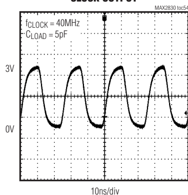
CLOCK OUTPUT
