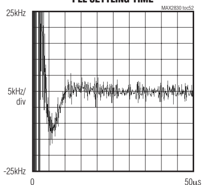
Rx-TO-Tx TURNAROUND PLL SETTLING TIME
