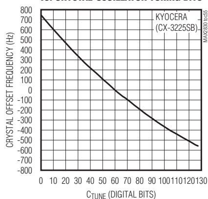
CRYSTAL-OSCILLATOR OFFSET FREQUENCY vs. CRYSTAL-OSCILLATOR TUNING BITS
