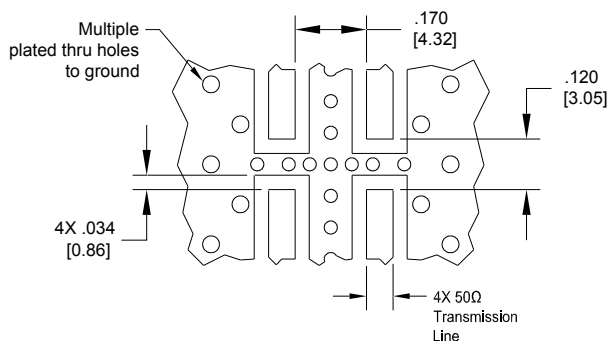
Dimensions are in Inches [Millimeters] X3C09P1-05S Mounting Footprint
