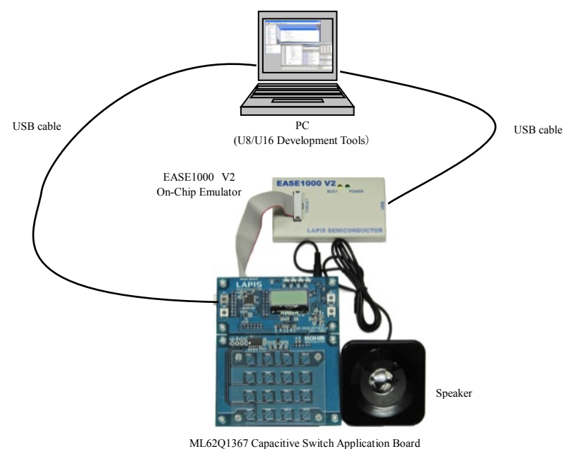
Figure 5 Use with the U8/U16 Development Tools configuration
